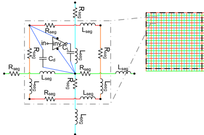
Fig. 2. In order to facilitate the P/G network analysis, each wire segment is modeled as a chain of L-type RLC equivalent circuits. An inverter with a capacitance load is used to imitate the core logic. A decap is connected to the intersection points on the vdd/vss grids.
