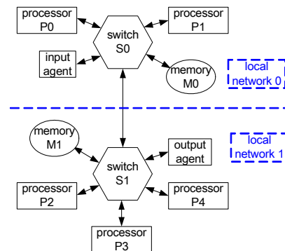
Figure 4. SoC architecture using application-specific NoC
